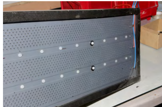
ESL 57 series production, rubber frame for Q57 tweeter
